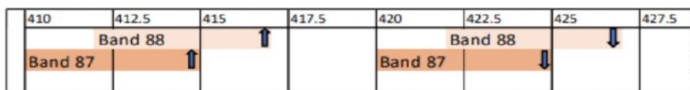
Figure 1: Two 3GPP band plans (87 and 88) for 410 MHz to 430 MHz band 100 .
