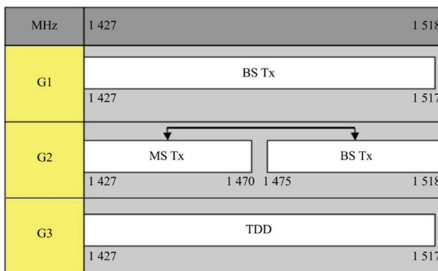
Figure 1: Channel arrangements for IMT1500 (Source ITU)
